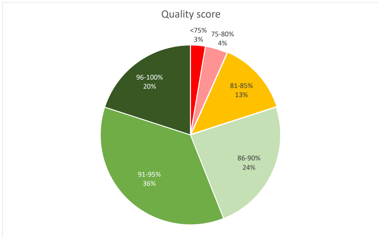
Figure 109: Quality score
