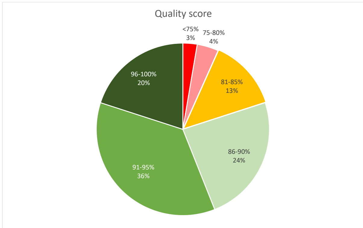
Figure 60: Quality score
